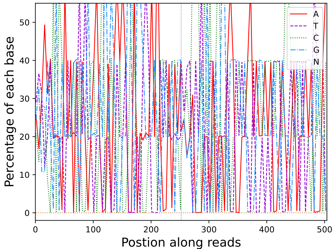
Base percentage along reads (R20204)
